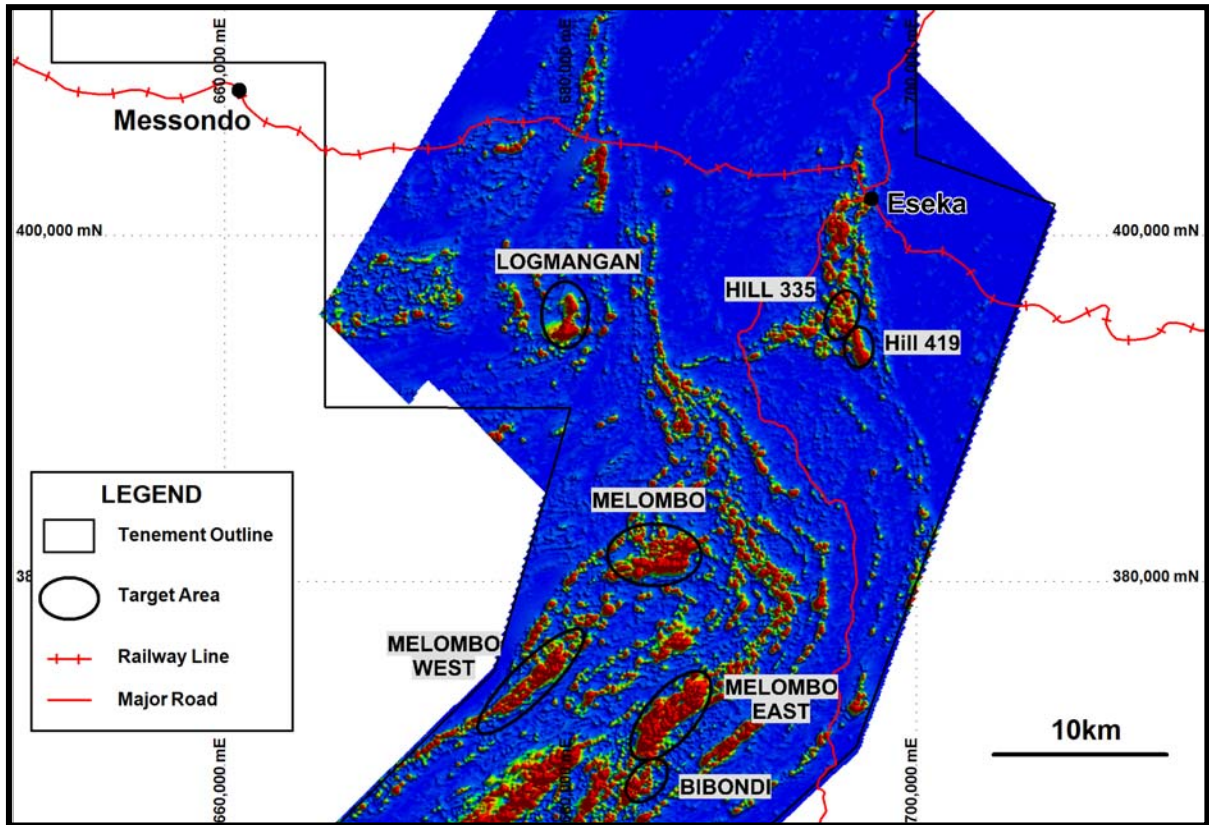
Figure 1: Ngovayang Project Drill Targets over Aeromagnetic Image (Analytical Signal of Total Magnetic Intensity)
