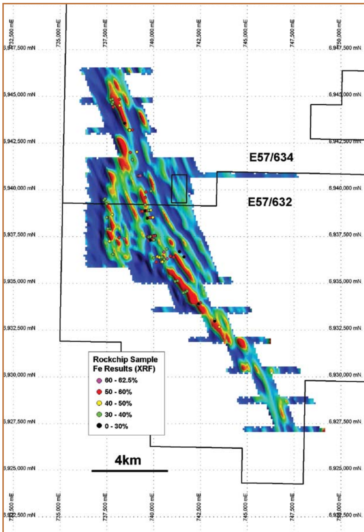
Figure 6: Woodley Residual Gravity Image with Rockchip Iron Sample Results
