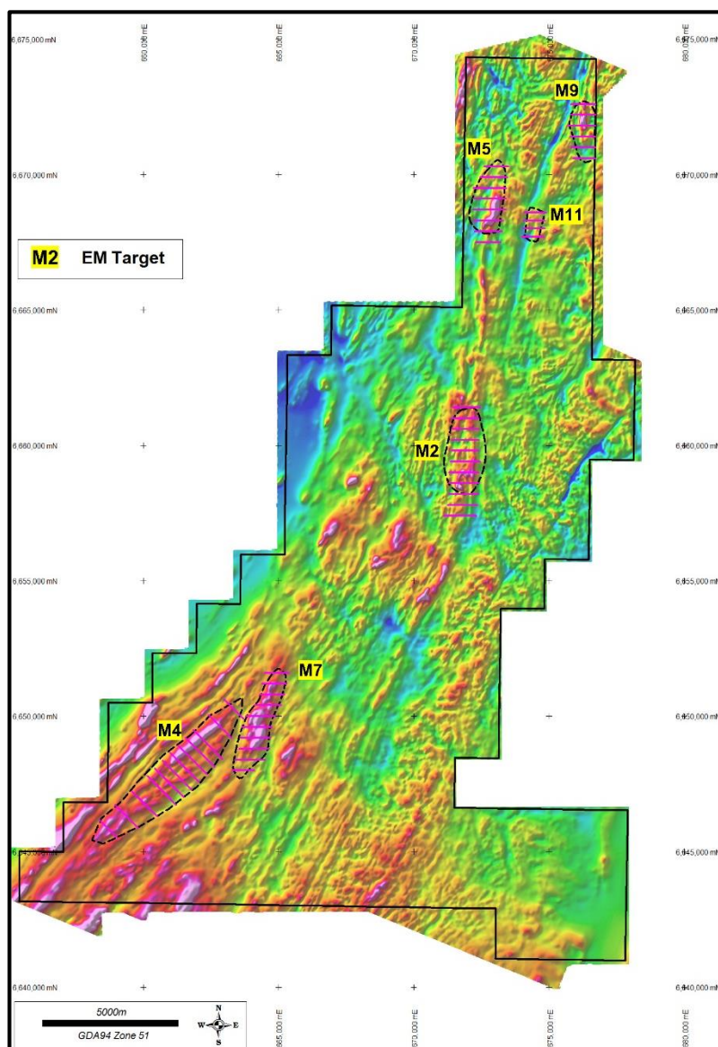
Figure 1: Targets tested with MLEM on aeromagnetic image
