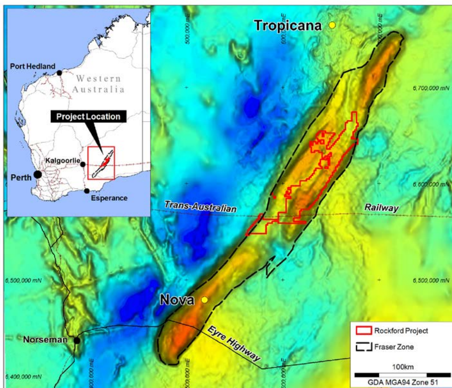
Figure 1: Rockford Project Location on Regional Gravity Image
