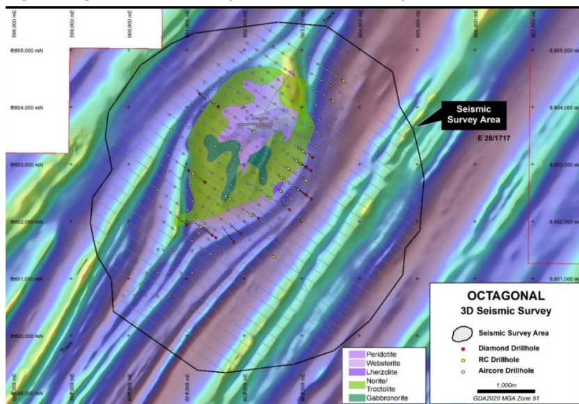
Fig.1. Octagonal Intrusive Complex with Seismic Survey Area
