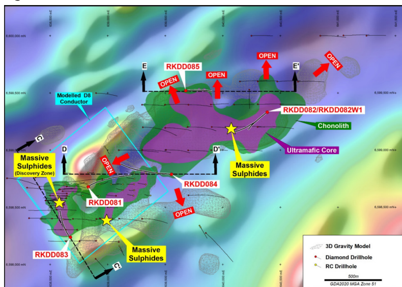
Fig.4. Mawson chonolith with diamond drillholes
